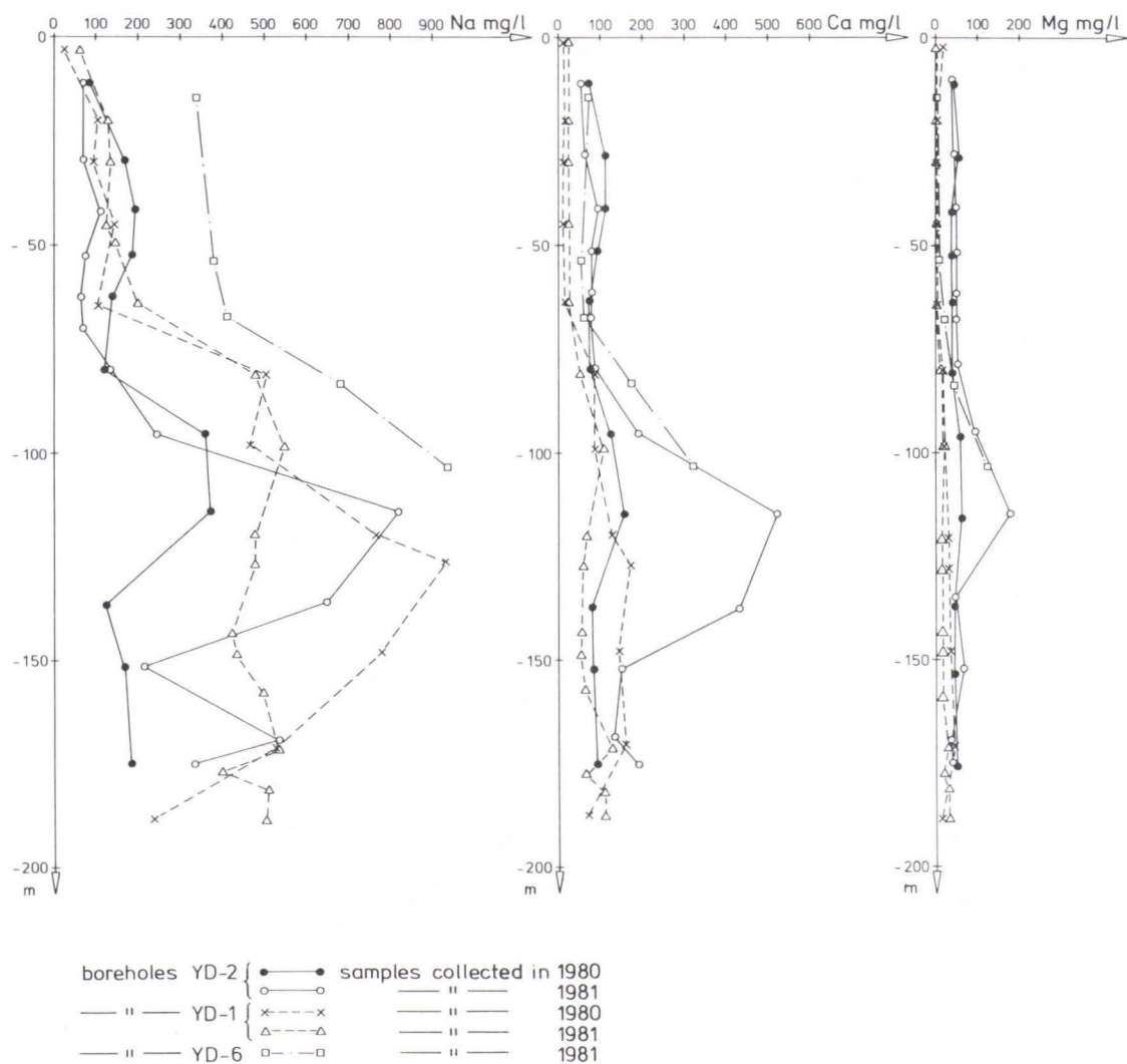
Fig. 8. \text{Na}^+ , \text{Ca}^{2+} and \text{Mg}^{2+} -ion content in the ground water of Olkiluoto.
