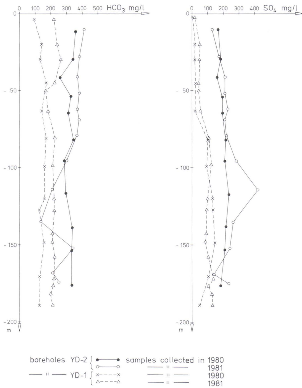
Fig. 7. \text{HCO}_3^- and \text{SO}_4^{2-} -ion content in the ground water of Olkiluoto.
