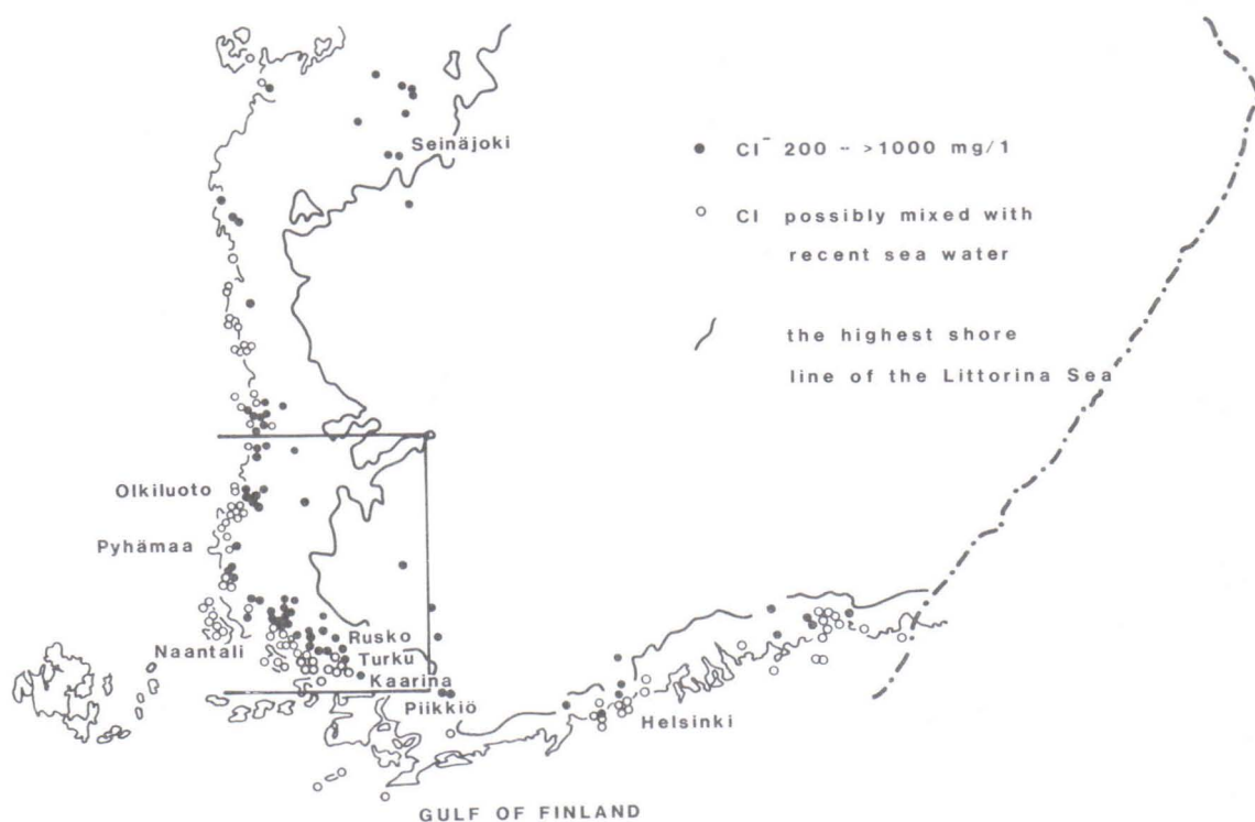
Fig. 10. Some wells with fresh and saline water in the coastal area and the highest shore line of the Littorina Sea. Some of the locations mentioned in Table 1, are presented along with the border of the study area (after Ehlers & Lahermo 1981).
